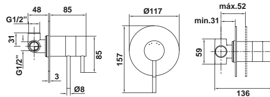
Concealed thermostatic shower mixer
