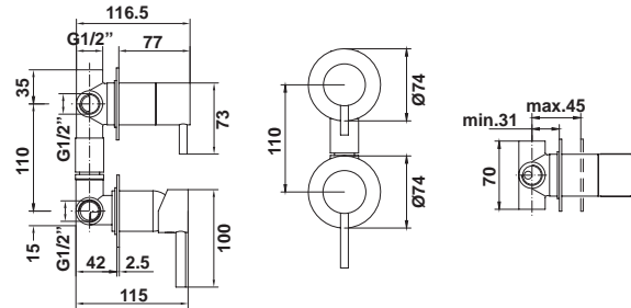
Built-in bath / shower mixer (3 outlets)
